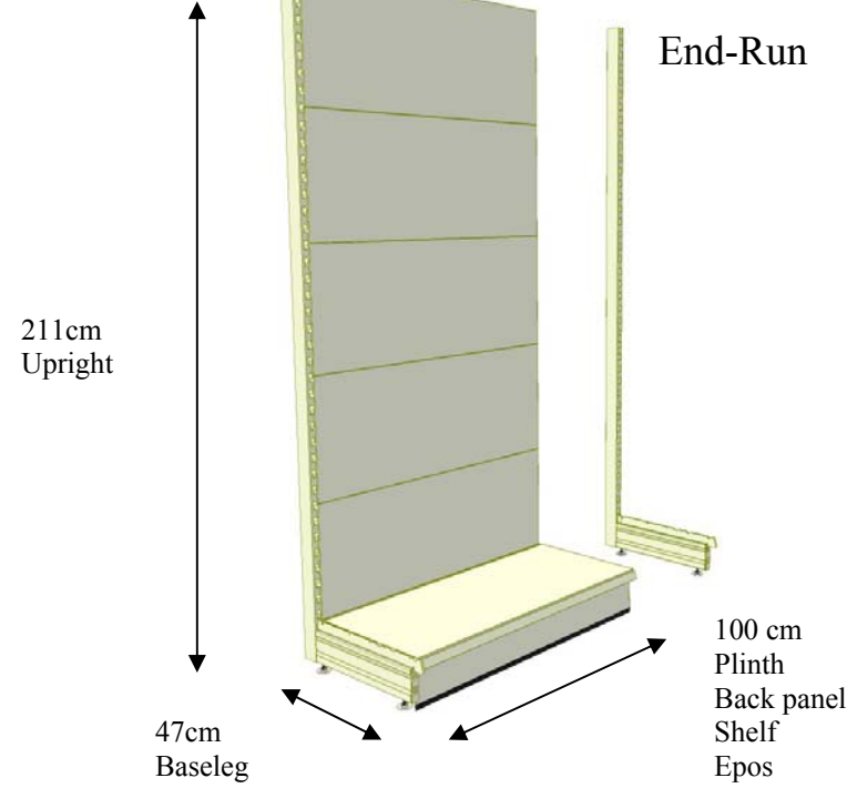
Shop Shelving Wall Bay
